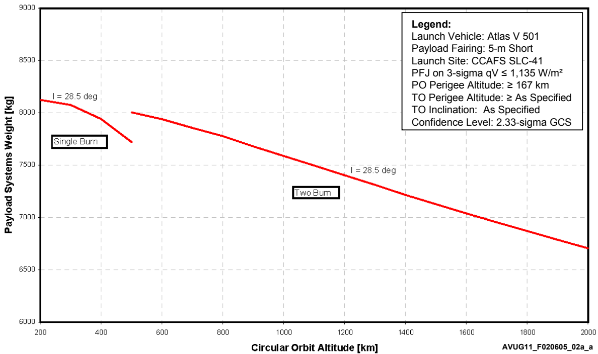
Figure 2.6.5-2a: Atlas V 501 Low Earth Orbit Performance — CCAFS
