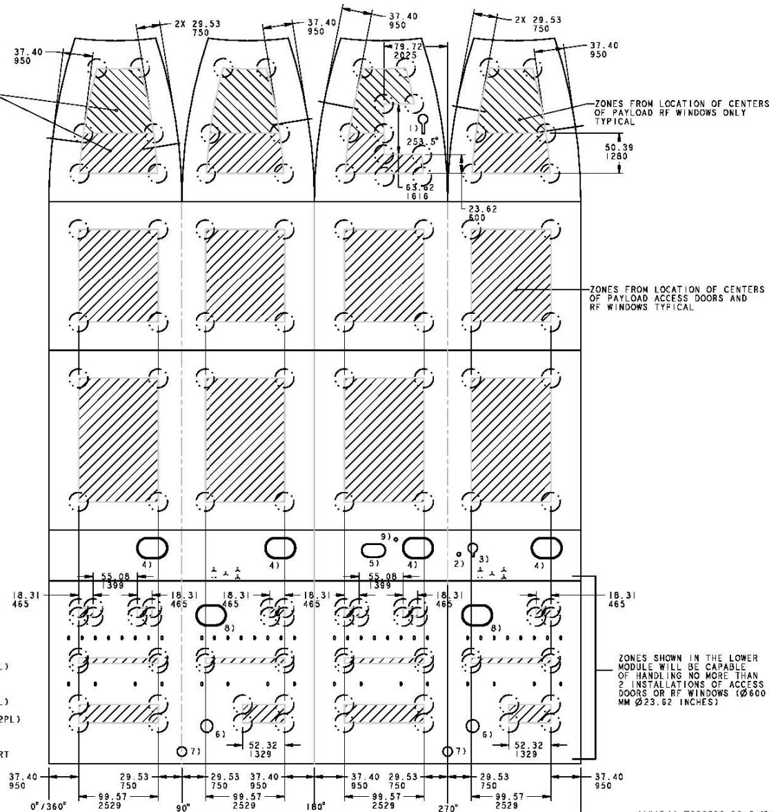
Figure 6.2.3-3: Atlas V 5-m Long PLF Mission Specific Access Door Allowable Locations (2 of 2)
