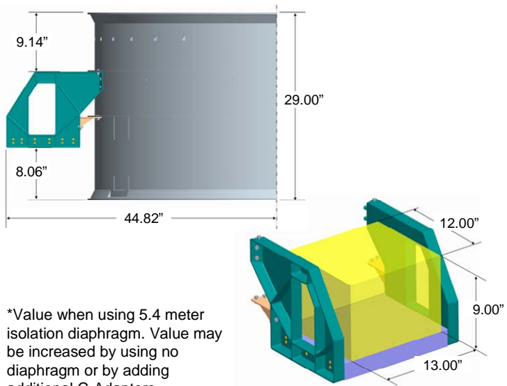
Figure 9.1.4-1: CAP Location and Volume
