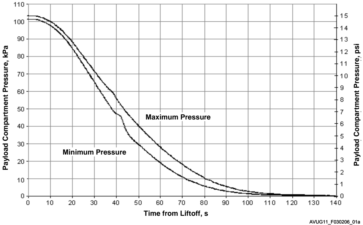
Figure 3.2.6-1: Typical Static Pressure Profiles inside the EPF for Atlas V 431
