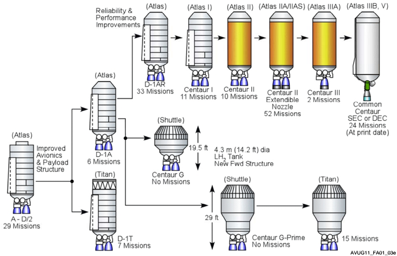
Figure A.1-3: Centaur Evolution Accommodates Boost Vehicle Performance and Reliability
