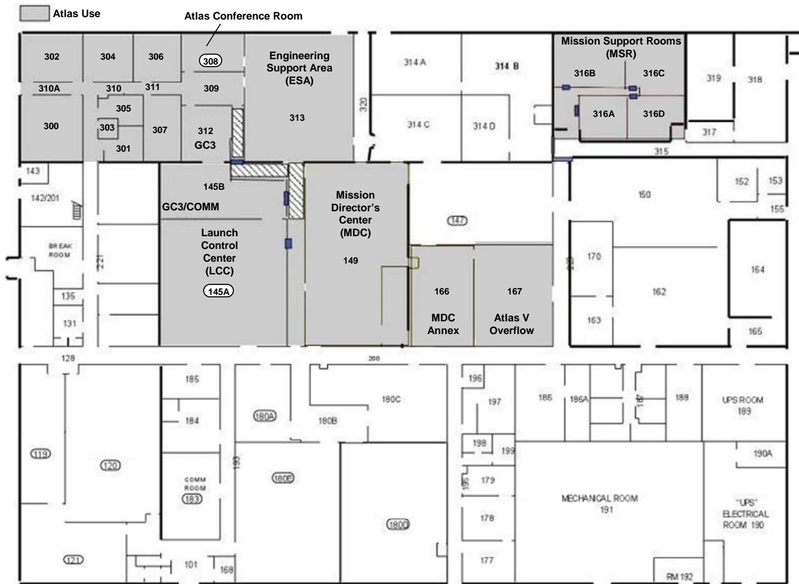
Figure 7.2.4-1: Atlas RLCC Area within Building 8510
