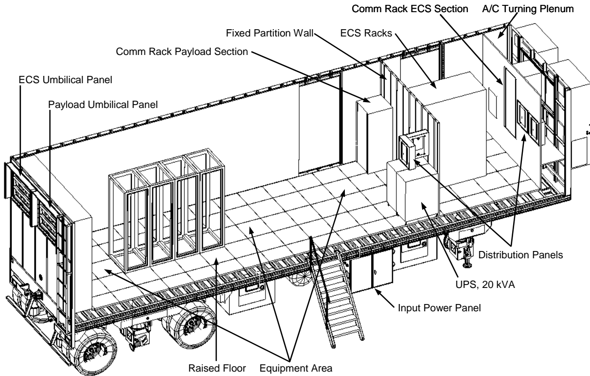
Figure 7.1.3.2-1: Payload Van
